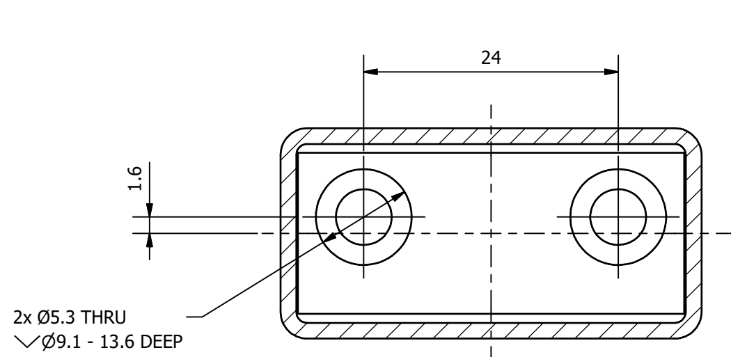
SECTION A-A MOUNTING DETAIL
